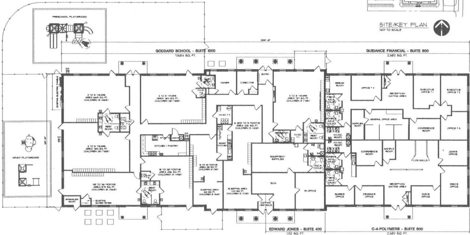
BUILDING 'A' TENANT LEASE PLAN 1/8" = 1'-0"
